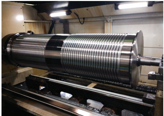
WHEEL & ROPE DRUM
